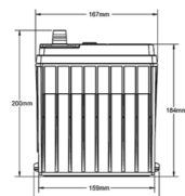
ODX-AGM34R RIGHT POSITIVE SAE TERMINALS
