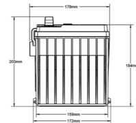
ODX-AGM34/78 LEFT POSITIVE DUAL TERMINALS (SAE & SIDE)
