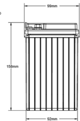
ODS-AGM16B LEFT POSITIVE FRONT FEMALE CONNECTION
