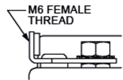
ODS-AGM16B LEFT POSITIVE FRONT FEMALE CONNECTION
